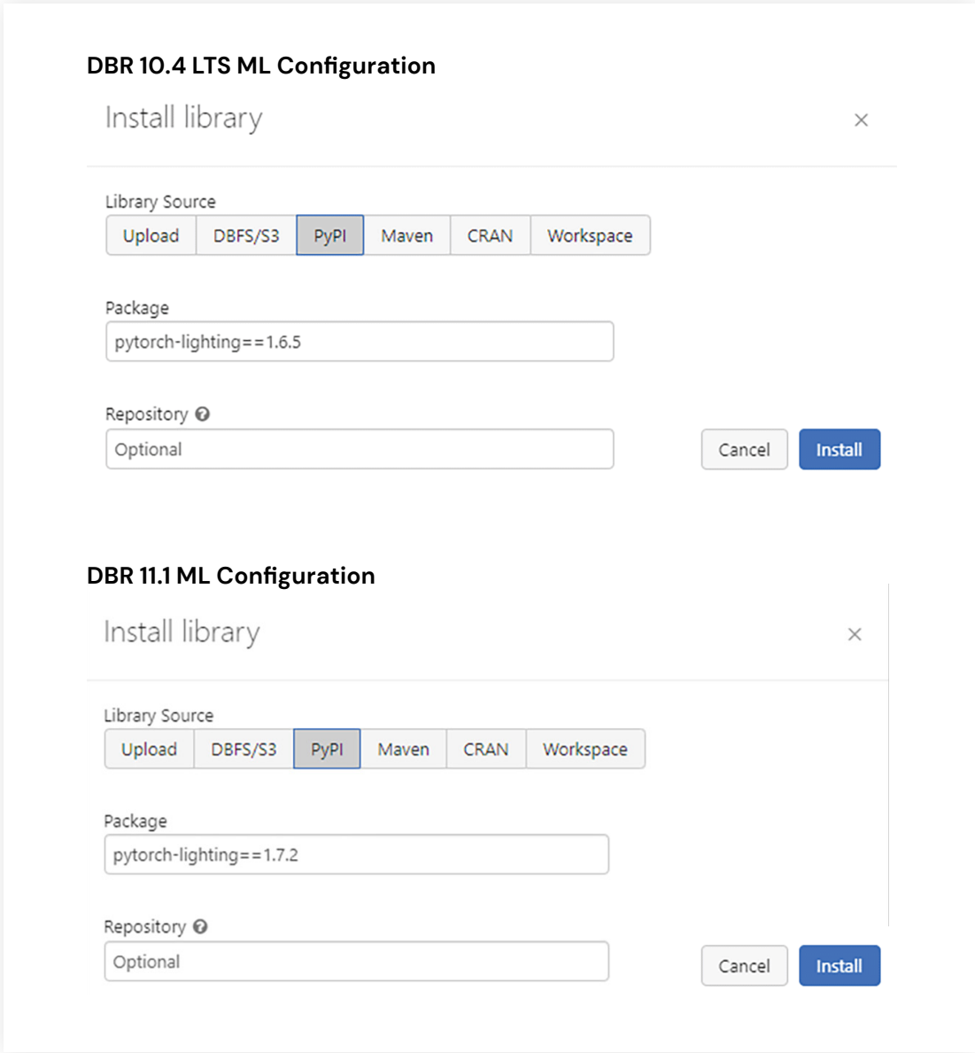
Figure 1: Library configuration
