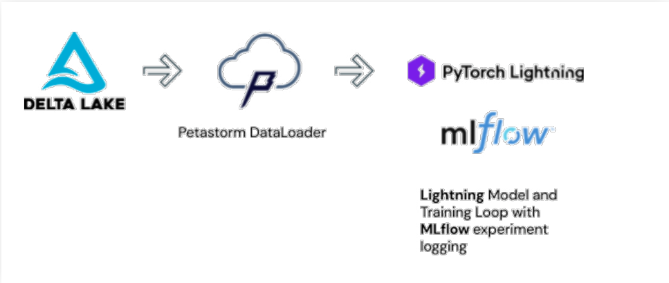
Figure 2: Key components
