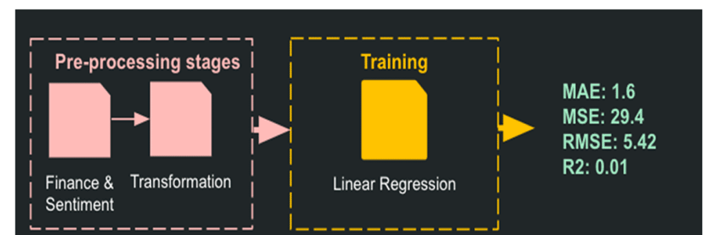
Figure 6: Correlation model pipeline
