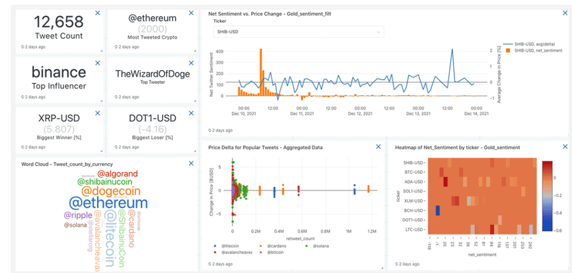
Figure 7: Overview Dashboard View with top level statistics
