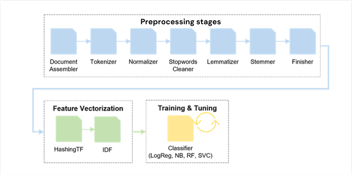
Figure 5: Machine learning model pipeline
