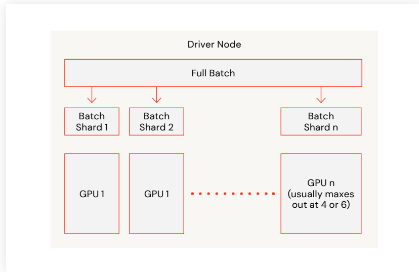
Figure 4: Single-node scaling
