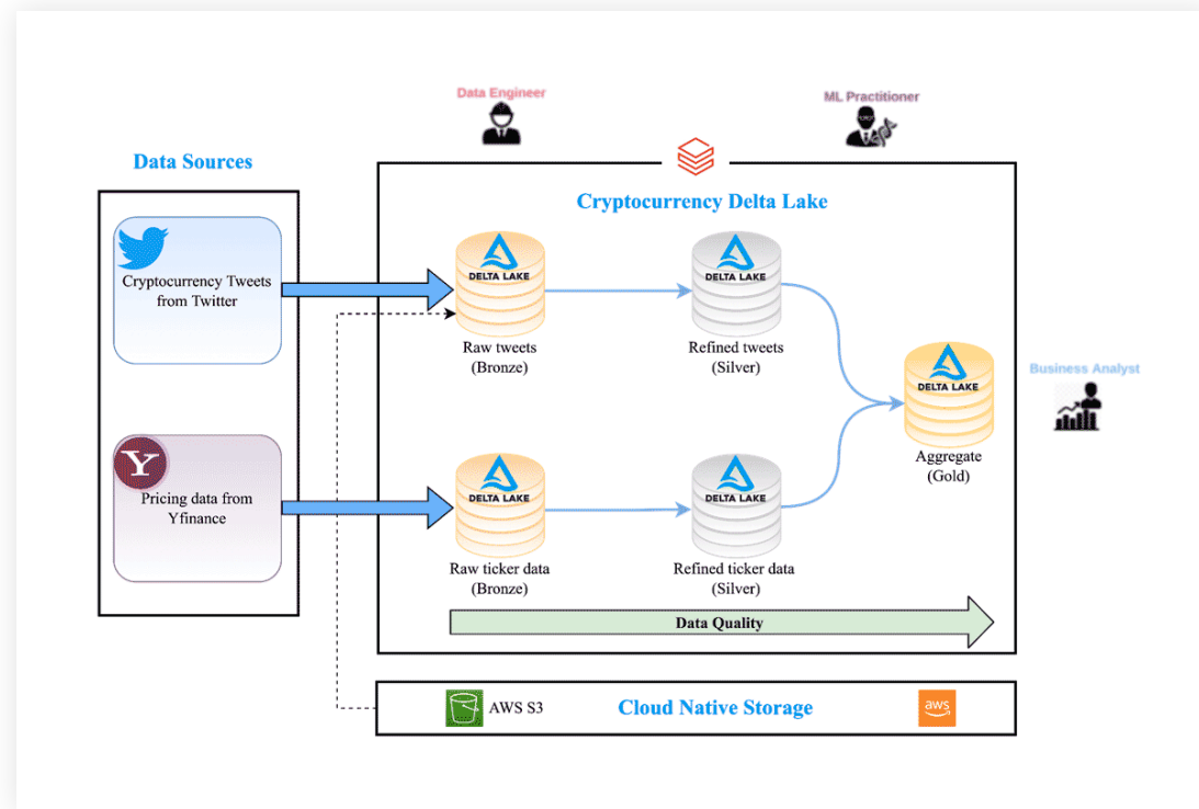
Figure 1: Crypto Lake using Delta
