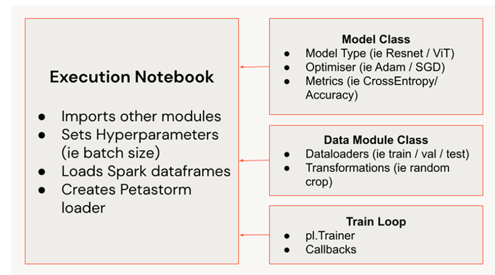
Figure 3: Code layout
