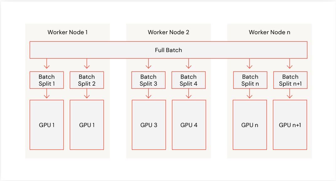
Figure 5: Multi-node scaling
